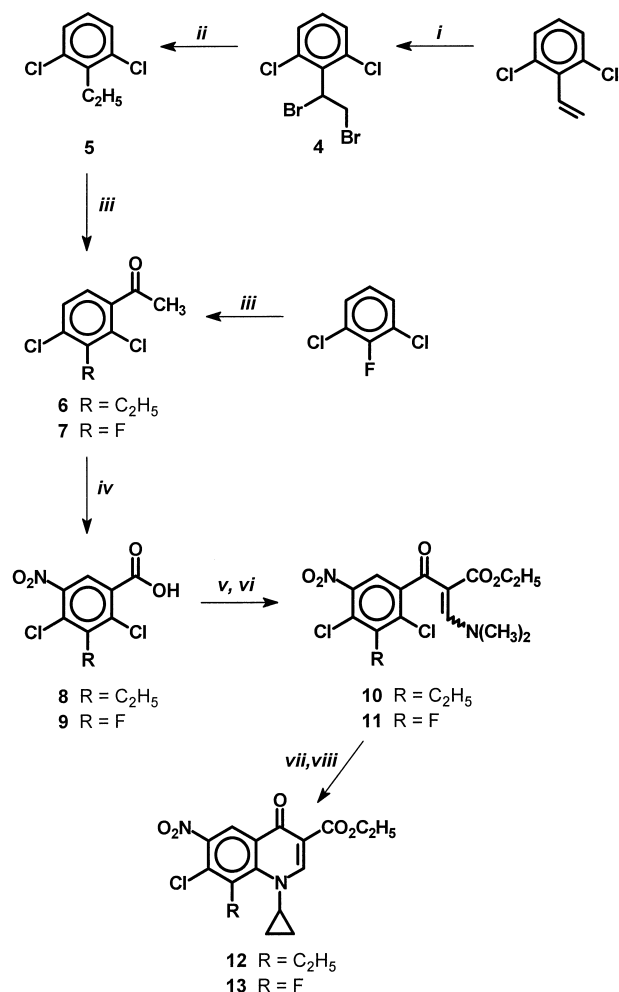
Scheme 1. Reagents: (i) Br 2 , CHCl 3 , 5°C; (ii) NaBH 4 , DMSO, 60°C; (iii) CH 3 COCl, AlCl 3 ; (iv) 90% HNO 3 , 98% H 2 SO 4 ; (v) SOCl 2 reflux; (vi) (CH 3 ) 2 NCH=CHCO 2 C 2 H 5 , Et 3 N, toluene, 90°C; (vii) c -PrNH 2 , EtOH/Et 2 O; (viii) KF or K 2 CO 3 , DMF, 160°C.
