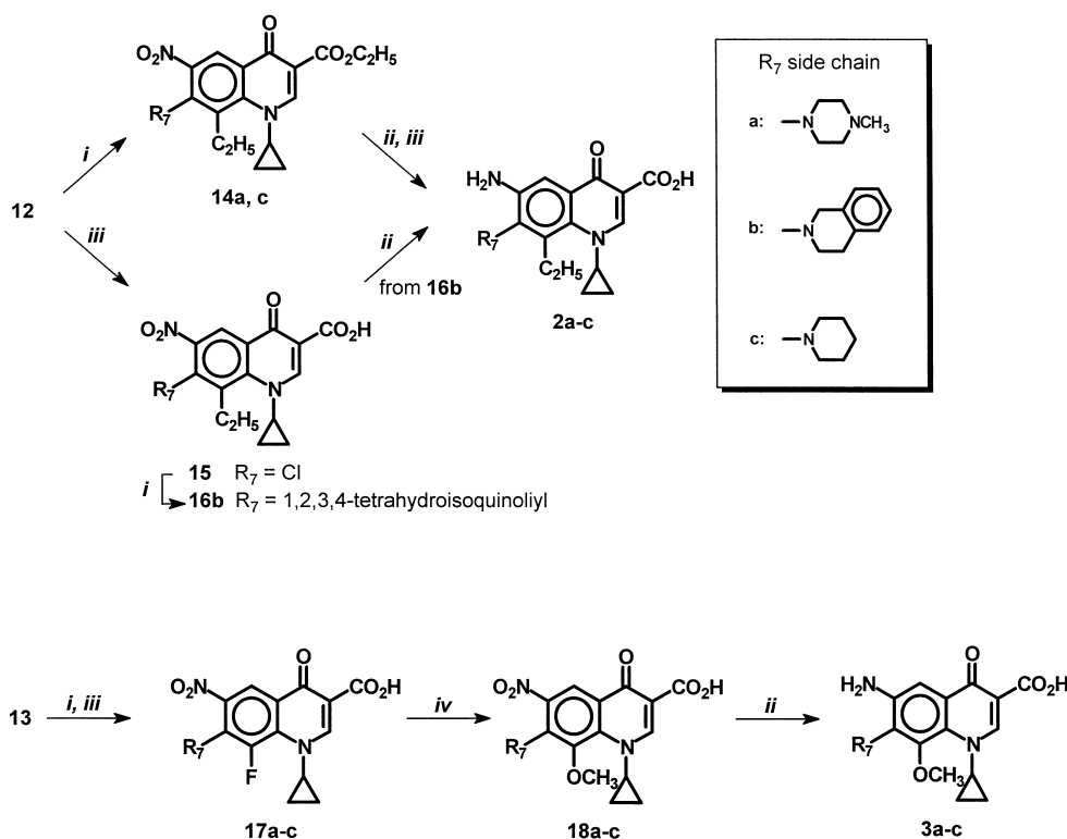
Scheme 2. Reagents: (i) R 7 H, CH 3 CN, reflux; (ii) H 2 , Raney-Ni, DMF or CH 3 OCH 2 CH 2 OH; (iii) 6 N HCl, EtOH, reflux; (iv) CH 3 ONa, CH 3 OH/DMF, 80°C.
